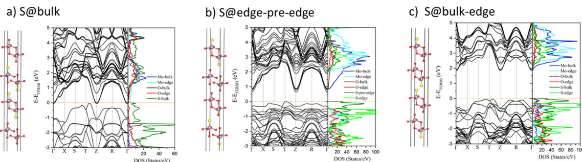
Fig. 5 Optimized structures, electronic band structures and PDOS of 4L MoO 3.5 O 2.5 ( x_s = 16.66\% ) for 3 different S substitution positions calculated by using HSE06: (a) inside the bulk only, (b) at edge and pre-edge, (c) at edge and in the bulk. The Fermi level is set to zero. The corresponding structures, band structures and PDOS for these systems are also reported in Fig. S3 and S5 (ESI † ) configurations h, i, and j, respectively.
