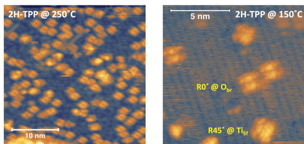
Fig. 20 Left: STM image (PtIr tip) of ~0.2 ML 2H-TPP molecules after self-metalation at 250 °C (+1.3 V, 96 pA). Right: A close-up view of isolated TPP molecules after self-metalation at 150 °C (+1.5 V, 40 pA).
