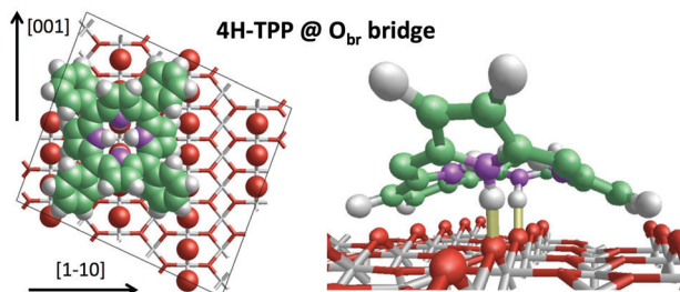
Fig. 5 Left: Top view of the 4H-TTP equilibrium configuration; the protruding O_{br} atoms (in red) have been enlarged; nitrogen, carbon and hydrogen atoms are painted in purple, green and white, respectively. Right: Perspective view of the 4H-TTP molecule, where the two hydrogen bonds N-H \cdots O_{br} are highlighted with yellow sticks. Adapted from ref. 45 with permission from the PCCP Owner Societies, Copyright 2015.
