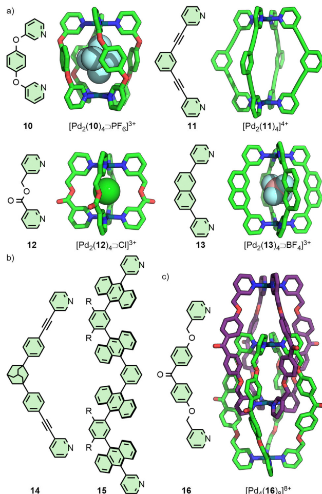
Fig. 3 (a) Bis-3-pyridyl ligands 10 – 13 and their \text{Pd}_2\text{L}_4 assemblies (SCXRD structures). Larger organic ligands (b) 14 and 15 also assemble into \text{Pd}_2\text{L}_4 cages, whilst (c) 16 , in the presence of suitably sized anions ( \text{A}^- ), yields the quadruply-interlocked metallo-catenane [\text{Pd}_4(\text{16})_8]^{8+} (SCXRD structure – encapsulated anions not shown).
