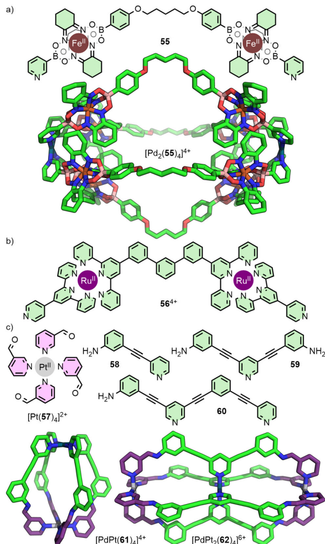
Fig. 11 Kinetically stable metallo-ligands such as (a) Fe(II)-clathrochelate 55 (SCXRD structure), and (b) bis-Ru(II) 56 4+ , each assemble with Pd(II) to give symmetrical \text{Pd}_2\text{L}_4 systems. (c) In contrast, the use of a subcomponent self-assembly strategy has allowed \text{M}_2\text{L}_4 and \text{M}_3\text{L}_4 cages (SCXRD structures) to be accessed in which Pd(II) and Pt(II) ions occupy distinct structural sites within these architectures, despite both residing in tetrapyrrolyl coordination environments.
