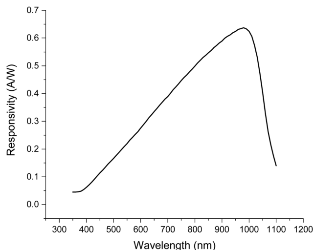
Fig. 4 Typical SRS detector responsivity vs. wavelength (FDS1010 silicon photodiode, Thorlabs). 30 Typical wavelengths used are 1000–1100 nm for the Stokes and 700–900 nm for the pump beams.
