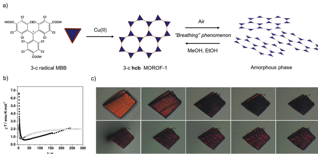
Fig. 4 (a) Schematic representation of the formation of hcb MOROF-1 using the 3-c PTMTC and Cu(II), and its breathing behaviour. (b) Value of \chi T as a function of the temperature for MOROF-1 (filled circle, MOROF-1; open circle, evacuated and amorphous MOROF-1 phase). (c) Breathing phenomenon of a single crystal of MOROF-1 when exposed to the air (top) and re-exposed to ethanol liquid (bottom). (b and c) Adapted from ref. 69. Copyright 2003 Nature Group.
