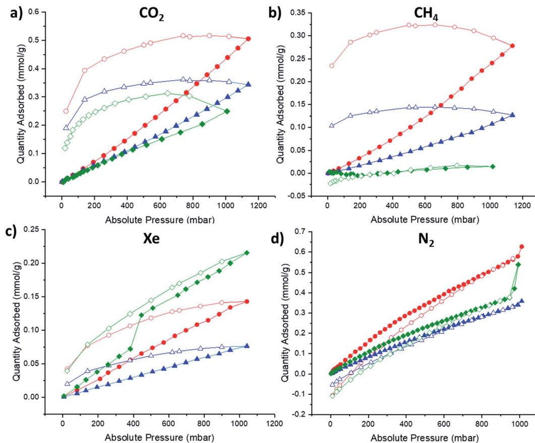
Fig. 5 Adsorption (filled) and desorption (empty) isotherms for RCC3-S (green), a_g RCC3-S (red), a_{fg} RCC3-S (blue): (a) \text{CO}_2 , 273 K; (b) \text{CH}_4 , 273 K; (c) Xe, 273 K; (d) \text{N}_2 , 77 K.
