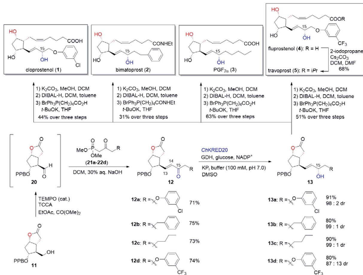
Fig. 5 Completion of the chemoenzymatic total synthesis of cloprosteno1 (1), bimatoprost (2), PGF_{2\alpha} (3), fluprostenol (4), and travoprost (5).
