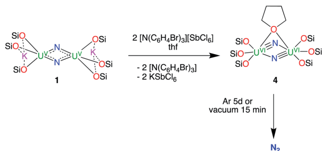
Scheme 2 Synthesis of complex [K 2 {U(OSi(O t Bu) 3 ) 3 } 2 (μ-N) 2 (μ-thf)], 4 and its decomposition.
