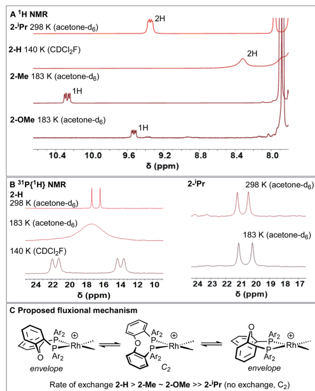
Fig. 5 (A) Low-field ( \delta 7.8–10.5) region of the ^1\text{H} NMR spectra for the [Rh(DPEphos-R)(NBD)][ \text{BAR}^F_4 ] complexes showing the shifted signals (temperature and solvent as noted) (B) ^{31}\text{P}\{^1\text{H}\} NMR spectra for 2\text{-H} and 2\text{-}^1\text{Pr} at various temperatures. (C) Proposed fluxional process.
