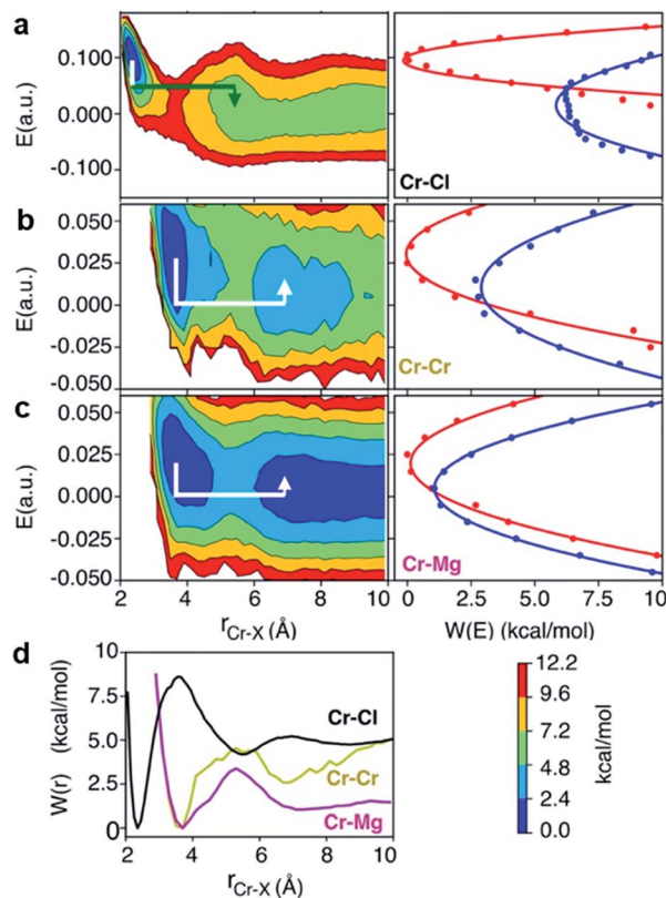
Fig. 7 2D free energy surfaces, involving Cr–Cl, Cr–Cr, Cr–Mg distance and electric field, E , experienced by (a) Cl - , (b) Cr, and (c) Mg with corresponding Marcus parabolas (solid lines are parabolic fits and dots are actual data), describing chloride exchange around Cr 3+ and dissociation of the Cr–Cr and Cr–Mg dimers. The lines with arrows are the Marcus pathways showing how reorganization of ionic media causes electric field rearrangement and drives the exchange and dissociation events. (d) The corresponding 1D free energy profiles.
