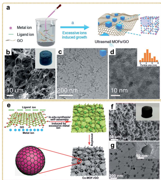
Fig. 4 (a) Illustration of the synthesis process of the PB/GO. (b) SEM image and (c and d) TEM images of the PB/GO aerogel. The inset of (b) is a photograph of the monolithic PB/GO aerogel. The inset of (d) is a histogram of the size distribution of PB nanoparticles. Reproduced with permission from ref. 39. Copyright 2020, Wiley-VCH. (e) Schematic illustration of the preparation of the Co-MOF-rGO hybrid. (f) SEM image, and (g) TEM images of the Co-MOF-rGO hybrid. The inset of (f) is a photograph of the monolithic Co-MOF-rGO aerogel. Reproduced with permission from ref. 40. Copyright 2020, American Chemical Society.
