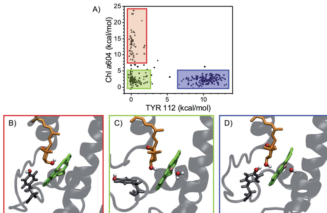
Fig. 6 The N1 binding pocket assumes different conformations. (A) Electrostatic interaction energy of N1 neoxanthin of LHCII with either TYR112 (x-axis) or Chl a604 (y-axis). Three different clusters of data points (each point represents a single MD snapshot) can be visualized in the scatter plot, representing either no strong interaction (enclosed in the green rectangle), preferential interaction with Chl a604 (red) or preferential HB to TYR112 (blue). The latter cluster is also the most abundant. (B–D) Conformations of the N1 binding pocket characterized by distinct interaction patterns and corresponding to three MD snapshots representative of the clusters shown in (A), with the same color code adopted for the surrounding rectangles. Neoxanthin is shown in orange, Chl a604 in green, TYR112 in gray, and the protein in transparent gray. The water molecule coordinating Chl a604 is also shown, if present. The polar oxygen and hydrogen atoms are highlighted in red and white, respectively, whereas the Mg of Chl a604 is highlighted in pink. In (B), the –OH group of neoxanthin interacts strongly with the Mg of Chl a604, which lacks the coordinating water molecule. In (C), neoxanthin shows weak interactions with both Chl a604 (which is coordinated by a water molecule) and TYR112. In (D), neoxanthin forms a strong HB with TYR112.
