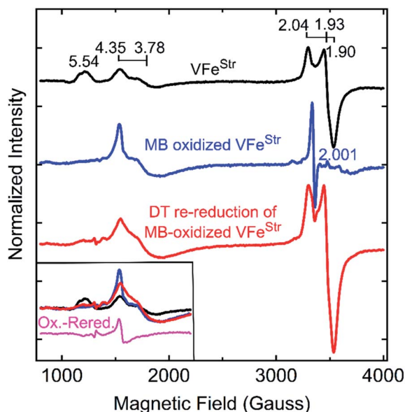
Fig. 4 X-band EPR spectra of oxidized VFe proteins. Shown is the resting state \text{VFe}^{\text{Str}} in MOPS buffer with 20 mM DT (black trace), methylene blue (MB)-oxidized \text{VFe}^{\text{Str}} after 15 min incubation at room temperature in MOPS buffer without DT (blue trace), and 20 mM DT re-reduced \text{VFe}^{\text{Str}} after being oxidized by MB for 15 min (red trace). The MOPS buffer was 100 mM, pH 7.3, with ca. 150 mM NaCl. The final \text{VFe}^{\text{Str}} concentration was 50 \mu\text{M} in all samples. The inset in the left bottom corner presents an overlay of the low field region of the spectra from three spectra and the spectra difference (magenta trace) between the MB-oxidized sample and DT re-reduced sample after MB oxidation. EPR conditions are the same as those in Fig. 3.
