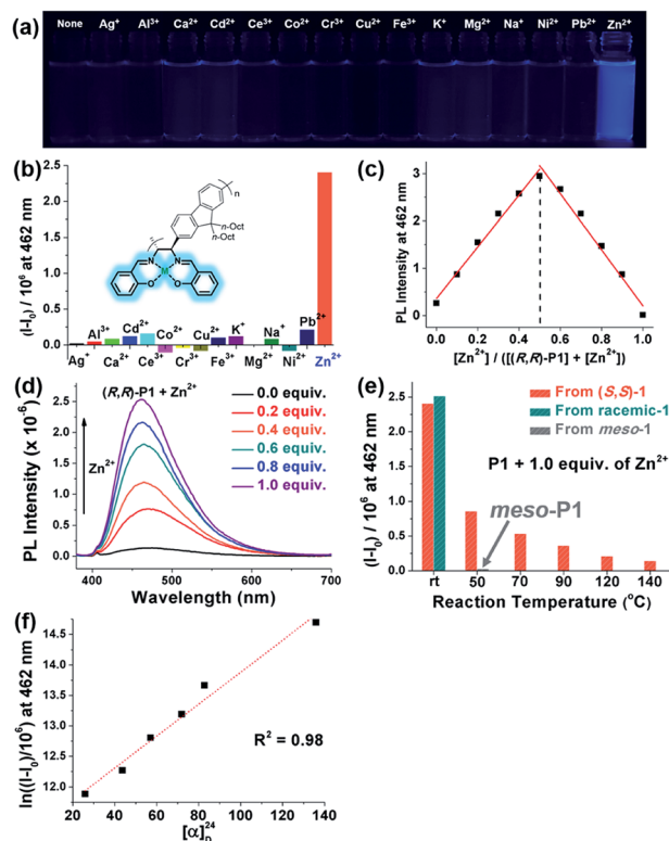
Fig. 6 Metal sensing experiments using P1 in THF : H 2 O = 9 : 1 (v/v) solution (10 \mu M) at 298 K. (a) Photoluminescence of ( R,R )- P1 solution in the absence or presence of 1.0 equiv. of various metal cations under 365 nm UV irradiation. (b) Emission changes of ( R,R )- P1 in the presence of 1.0 equiv. of various metal cations. (c) Job plot of ( R,R )- P1 vs. Zn 2+ (total concentration = 20 \mu M). (d) Emission spectra of ( R,R )- P1 with increasing amounts of Zn 2+ (0.0–1.0 equiv.). (e) Effect of polymerization temperature on the Zn 2+ sensing performance of P1 . (f) Correlation between fluorescence enhancement ( I - I_0 ) and optical rotation ( [\alpha]_D^{24} ) of P1 .
