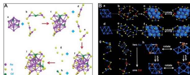
Fig. 14 Anatomy of the structure of (A) \text{Au}_{20}\text{Cd}_4(\text{SH})(\text{SR})_{19} and (B) \text{Au}_{26}\text{Cd}_4(\text{CHO})_{22} nanoclusters (reproduced from ref. 92 with permission from John Wiley and Sons, Copyright (2018) and ref. 93 with permission from the American Chemical Society, Copyright (2019)).
