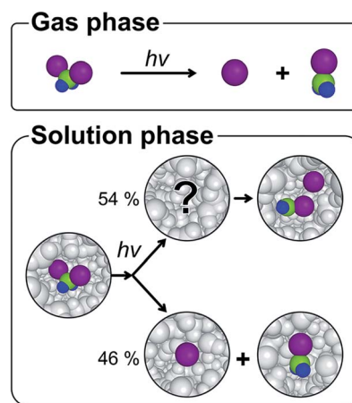
Fig. 1 The photodissociation dynamics of \text{CH}_2\text{I}_2 in the gas and solution phases. Whereas the products in the gas phase are \text{CH}_2\text{I}^{\cdot} and \text{I}^{\cdot} radicals ( \text{CH}_2\text{I}^{\cdot} + \text{I}^{\cdot} ), the \text{CH}_2\text{I} –I isomer is also observed in the solution phase. The green, blue and purple balls indicate carbon, hydrogen, and iodine atoms, respectively. Whereas the branching ratio into the \text{CH}_2\text{I} –I isomer and \text{CH}_2\text{I}^{\cdot} + \text{I}^{\cdot} of 54 : 46 and the molecular structure of the \text{CH}_2\text{I} –I isomer were determined in a previous TRXL study at a synchrotron, the exact structure of the precursor of the stable \text{CH}_2\text{I} –I isomer remained to be determined and was probed with femtosecond TRXL in this study.
