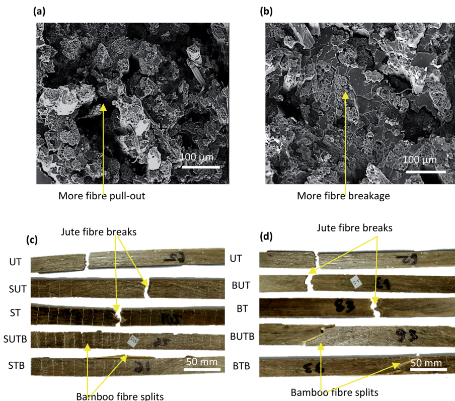
Fig. 6 SEM images of the fracture surfaces of (a) untreated (UT) and (b) stitched alkali-treated (ST) composites. Digital images of specimens after tensile testing: (c) stitched-preform-based and (d) sized-preform-based jute fibre composites.
