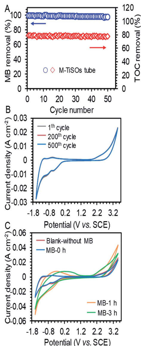
Fig. 3 (A) Stability performance of MB and TOC removal during 50 cycles of operation and (B) periodic CV tests in 0.5\text{ mol L}^{-1}\text{ Na}_2\text{SO}_4 with 50\text{ mg L}^{-1} MB solutions at a scan rate of 50\text{ mV s}^{-1} for the M-TiSO electrode. (C) CV curves in blank (without MB), untreated (0 h), and treated solutions (1 and 3 h) at a scan rate of 50\text{ mV s}^{-1} .
