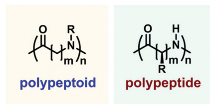
Fig. 2 Structures of a polypeptoid and polypeptide.
