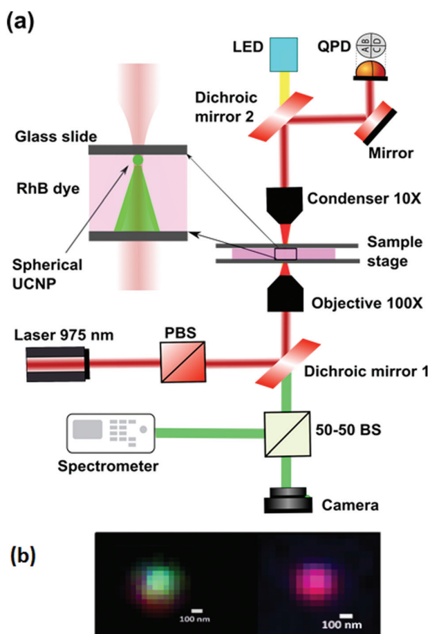
Fig. 3 (a) The schematic diagram for the experiment. 975 nm light is used to trap an UCNPs and the emission is used to perform absorption imaging (b) typical images of a 120 nm UCNPs in water (left) and in the presence of the dye (right), as recorded by the camera.
