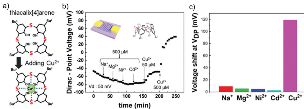
Fig. 11 2D electrical sensor based on graphene for the detection of Cu 2+ . (a) Chemical structure of thiocalix[4]arene receptors for the recognition of Cu 2+ ions. (b) Real-time detection of Cu 2+ via monitoring of the Dirac Point voltage of functionalized graphene TFTs (inset: device sketch). (c) Selective Cu 2+ sensing and device response in the presence of interfering cations. Adapted with permission from ref. 74 Copyright 2020 American Chemical Society.
