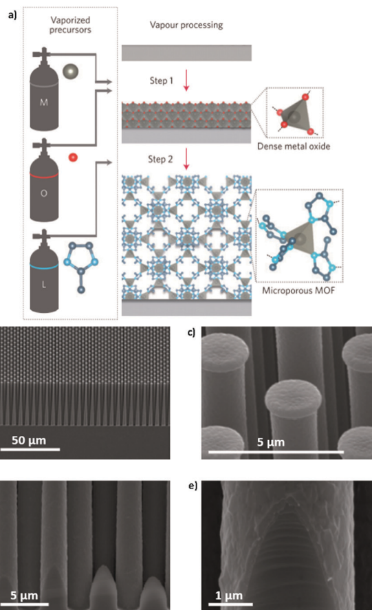
Fig. 10 (a) Schematic representation of the CVD route in two steps. Step 1: deposition of the oxide sacrificial layer; step 2: conversion of the metal oxide into a MOF thin film. (b and c) SEM images of a ZIF-8 coating on a silicon pillar array. (d and e) High-magnification SEM pictures of the homogeneous coverage at the base of the pillar, showing that the conformality typical of the ALD process is retained after the coordination replication reaction. Reproduced from ref. 63, copyright (2016), with permission from Elsevier.
