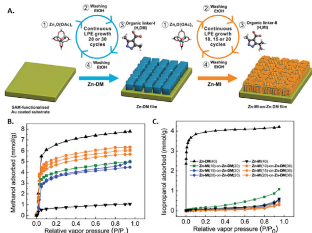
Fig. 17 Hierarchical structuring of MOF thin films on QCM substrates for selective adsorption. (A) Schematic illustration of the continuous stepwise LPE fabrication of heterostructured [Zn_4O(carboxypyrazolate)_3]_n thin films, wherein the core-layer MOF is composed of Zn-DM and the shell-layer MOF is composed of Zn-MI. Single-component (b) methanol and (c) isopropanol adsorption isotherms at 25 °C for Zn-MI, Zn-DM and various Zn-MI(x)-on-Zn-DM(y) heterostructured films using an environmental-controlled QCM. Note that x and y represent the number of deposition cycles for Zn-MI and Zn-DM, respectively. This figure was adapted with permission from J. Mater. Chem. A , 2015 , 3, 23385–23394. Copyright 2015, Royal Society of Chemistry.
