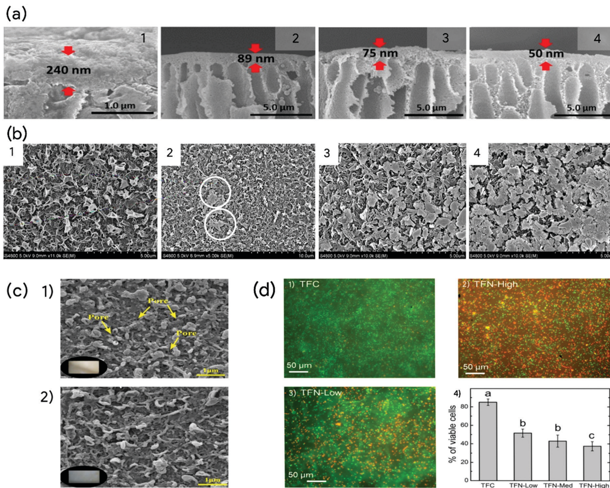
Fig. 2 (a) Cross-sectional SEM images of control and TFN membranes incorporated with 0.002 wt%, 0.003 wt% and 0.005 wt% mGO respectively (1–4), Adapted with permission. 54 Copyright 2019 Elsevier. (b) SEM surface morphologies of control and TFN membranes incorporated with 0.005 wt%, 0.02 wt% and 0.05 wt% MoS 2 respectively (1–4), Adapted with permission. 78 Copyright 2018 Elsevier. (c) SEM surface morphologies (1–2), of PA and 0.015 wt% Ti 3 C 2 T x incorporated PA15 membranes after chlorine exposure test, Adapted with permission. 16 Copyright 2020 Elsevier. (d) Epifluorescence microscopy images of E. coli cells on control TFC (1), TFN-Low (2) and TFC-High (3). Green and red colour represents live and dead cells, respectively. (4) Cell viability of adhered E. coli cells after 3 h of contact. Adapted with permission. 46 Copyright 2018 Elsevier.
