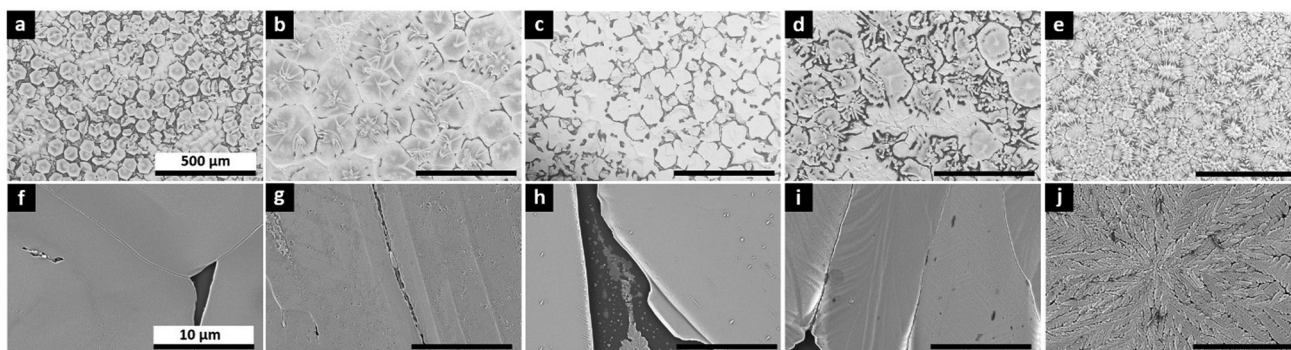
Fig. 2 SEM images of MAPb 0.5 Sn 0.5 I 3 with 0% (a; f), 0.1% (b; g), 0.2% (c; h), 1% (d; i) and 5% (e; j) F4TCNQ dopant, using an Everhart–Thornley detector with 100× magnification (a to e) and a Trinity detector with 5000× magnification collecting mostly secondary electrons (f to j). The scale bar is 500 μm for (a) to (e) and 10 μm for (f) to (j).
