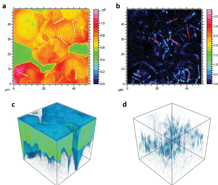
Fig. 3 TOF-SIMS 2D images of 1% doped MAPb 0.5 Sn 0.5 I 3 exhibiting the total signal (a) and the F signal (b). Each image is 50 × 50 μm and the color scale for each image shows the intensity in counts/pixel. The green area in panel (a) corresponds to uncoated glass substrate. White and red dotted lines are drawn as guide to the eye to show examples of grain boundaries visible in the total (a) and F (b) signals. TOF-SIMS 3D tomography rendering of the same dataset showing the signal coming from MA (MA: methylammonium), indicating the presence of the perovskite (c) and the F signal (d). Each 3D reconstruction is 50 × 50 × film thickness μm 3 .
