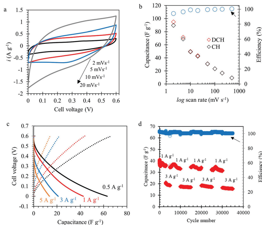
Fig. 6 Electrochemical performance of the symmetric device of Mo 1.33 CT z -cellulose composite electrodes (L-Mo 1.33 C-25% Cel symmetric device) in 1 M H 2 SO 4 solution: (a) cyclic voltammograms of the symmetric device at scan rates of 2, 5, 10 and 20 mV s -1 . (b) Variation of the charge-discharge capacitances with scan rates. (c) Potential capacitance profiles for the symmetric device under applied current densities of 0.5 (black), 1 (red), 3 (blue), and 5 (orange) A g -1 . (d) Variation of discharge capacitance with cycle number for the symmetric device at applied current densities of 1 and 3 A g -1 .
