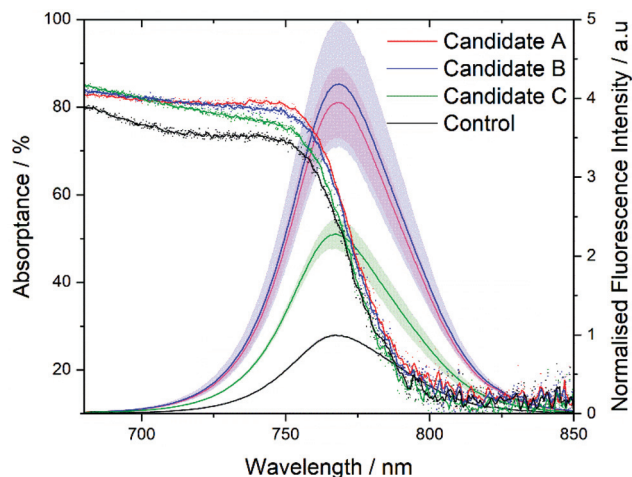
Fig. 5 Absorbance and photoluminescence – excitation wavelength ( \lambda_{\text{ex}} 450 nm) for each film manufactured in ambient conditions from the control and candidate solvents. Three films per solution were evaluated, 3 nm excitation and emission slit widths and repeat measurements under constant illumination were used to mitigate the effect of photo-brightening. All curves have been normalised to the maximum value of the control PL curve. The final ‘stabilised’ curve was used for each sample to create the average curve. The standard deviation of each sample set is displayed as the shaded region (film thicknesses were determined through profilometry with mean average values of: 366, 487, 492, and 365 nm for the control, A, B, and C).
