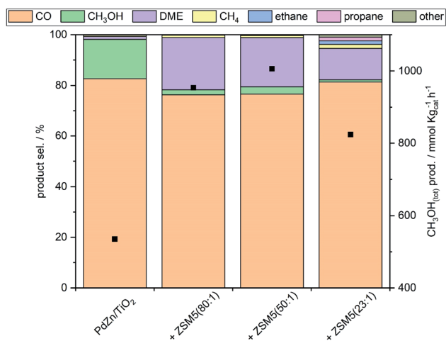
Fig. 3 CO, oxygenate and hydrocarbon selectivity and total \text{CH}_3\text{OH} productivity for \text{CO}_2 hydrogenation (20 bar, 270 °C, \text{CO}_2/\text{H}_2/\text{N}_2 = 1 : 3 : 1 ) over PdZn/TiO 2 and PdZn/TiO 2 -ZSM-5 hybrid catalysts.
