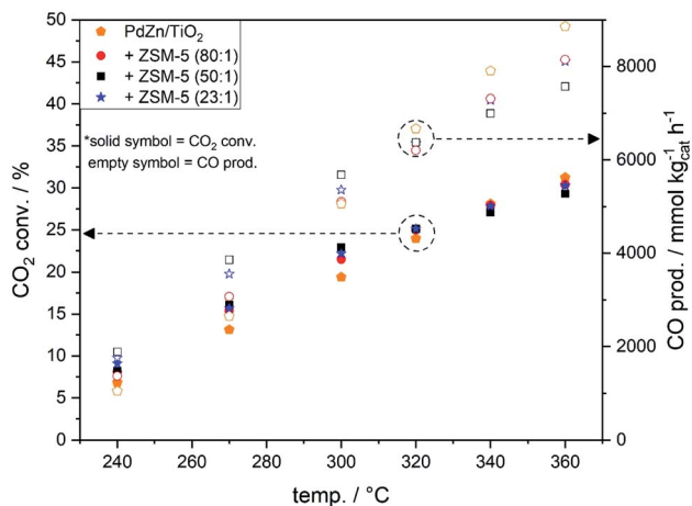
Fig. 2 \text{CO}_2 conversion and CO productivity over PdZn/TiO 2 and PdZn/TiO 2 -ZSM-5 hybrid catalysts during \text{CO}_2 hydrogenation (20 bar, 30 ml min -1 , \text{CO}_2/\text{H}_2/\text{N}_2 = 1 : 3 : 1 , 240–360 °C, 6 h dwell).
