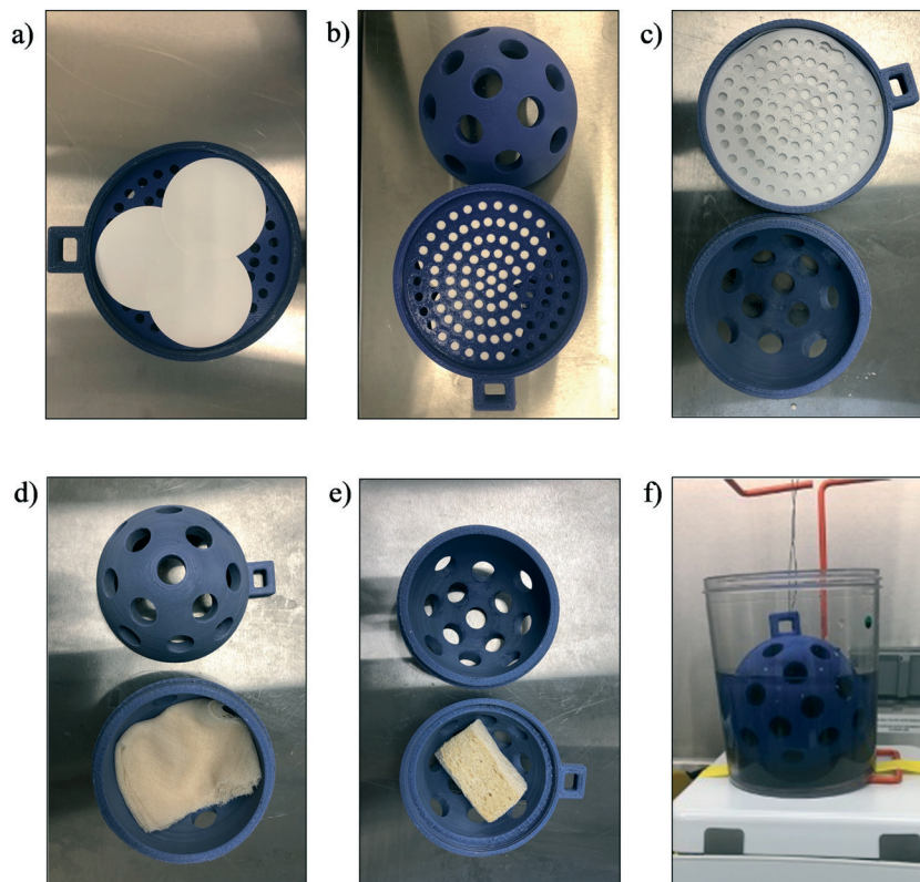
Fig. 1 Placement of different adsorbent materials inside the COVID-19 sewer cage (COSCa) passive sampler. a) Arrangement of three 4.7 cm electonegative filters; b) filters secured inside the COSCa insert; c) 9.0 cm filter inside a COSCa insert for field sample collection; d) gauze/cheesecloth and e) cellulose sponge placement inside the COSCa; and f) laboratory bench-scale COSCa passive sampling experimental set-up.
