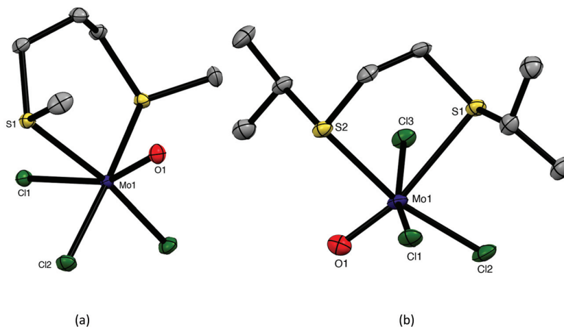
Fig. 1 Crystal structures of fac -[MoOCl 3 {MeS(CH 2 ) 3 SMe}] (a) and mer -[MoOCl 3 { t PrS(CH 2 ) 2 S'Pr}] (b) showing the atom numbering scheme. Ellipsoids are shown at 50% probability, hydrogen atoms omitted for clarity. Selected bond lengths (Å) and angles (°): (a) Mo1–Cl1 = 2.4540(2), Mo1–Cl2 = 2.3451(2), Mo1–Cl3 = 2.3451(4), Mo1–O1 = 1.674(1), Mo1–S1 = 2.5388(3), Cl1–Mo1–Cl2 = 94.52(2), Cl2–Mo1–Cl3 = 92.55(3), Cl2–Mo1–O1 = 101.87(4), Cl3–Mo1–O1 = 101.87(4), S1–Mo1–S1 = 97.95(2); (b) Mo1–Cl1 = 2.3578(8), Mo1–Cl2 = 2.3378(8), Mo1–Cl3 = 2.3618(7), Mo1–O1 = 1.671(2), Mo1–S1 = 2.8298(8), Mo1–S2 = 2.5665(7), Cl1–Mo1–Cl2 = 91.25(3), Cl1–Mo1–O1 = 98.99(8), Cl1–Mo1–Cl3 = 89.69(3), Cl2–Mo1–O1 = 98.99(8), S1–Mo1–S2 = 78.83(2).
