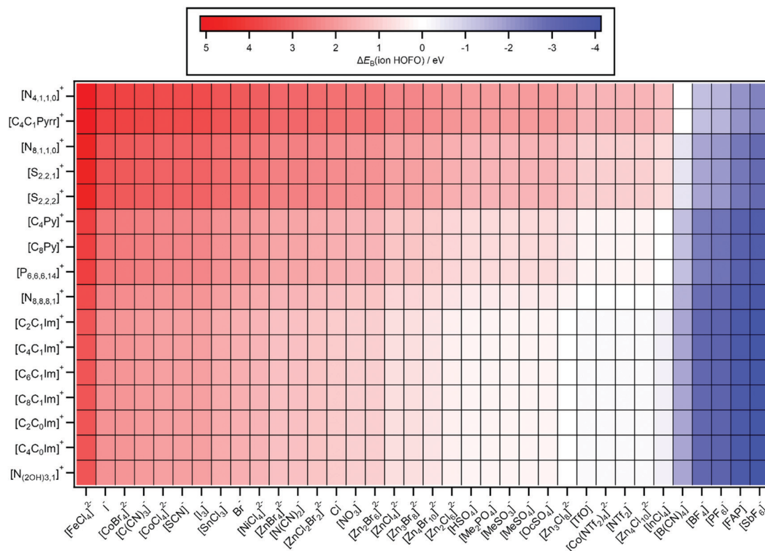
Fig. 7 Predicted \Delta E_B(\text{ion HOFO,pred.}) = E_B(\text{cation HOFO,pred.}) - E_B(\text{anion HOFO,pred.}) = E_i(\text{cation,pred.}) - E_i(\text{anion,pred.}) . The errors in \Delta E_B(\text{ion HOFO,pred.}) generally range from \pm 0.4 eV to \pm 0.6 eV.
