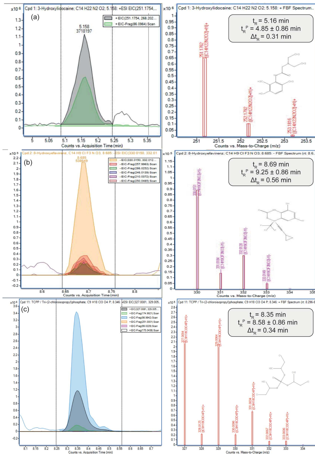
Fig. 3 Extracted ion chromatograms of (a) 3-hydroxyildocaine, (b) 8-hydroxyefavirenz and (c) TCPP in the passive sampler extracts. (Left) Extracted ion chromatograms of the [M + H]^+ (a and c) and [M - H]^- (b) ion and relevant fragments measured by DIA. Right: denotes the isotopic fit of the [M + H]^+ (a and c) and [M - H]^- (b) and matching predicted retention times.
