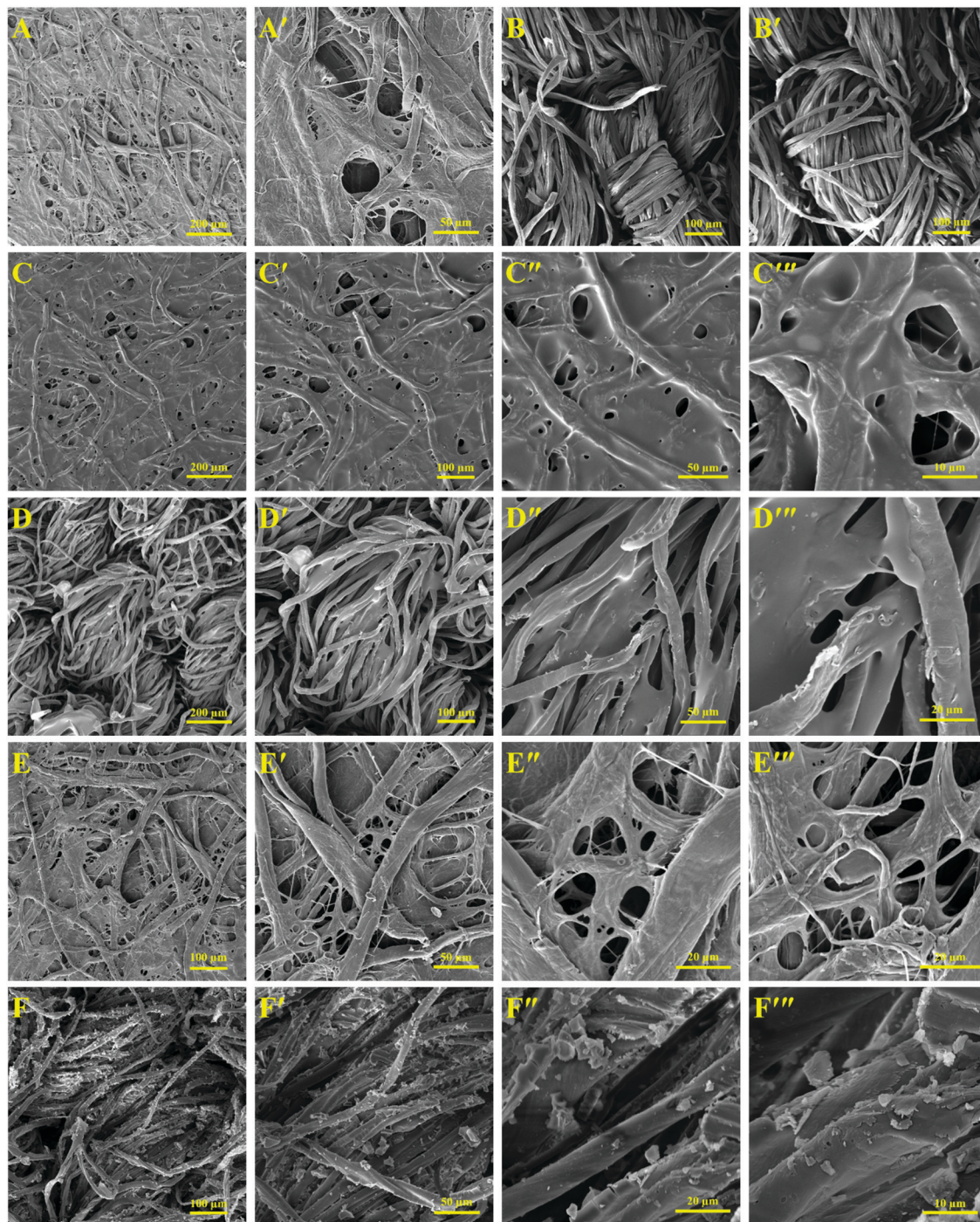
Fig. 9 SEM images of the impregnated cellulosic paper and tissue with the spiropyran-modified latex particles: (A and A') neat cellulosic paper, (B and B') neat cotton tissue, (C–C''') impregnated cellulosic paper with PBA-SP, (D–D''') impregnated cotton tissue with PBA-SP, (E–E''') impregnated cellulosic paper with PMMA-SP, and (F–F''') impregnated cotton tissue with PMMA-SP.
