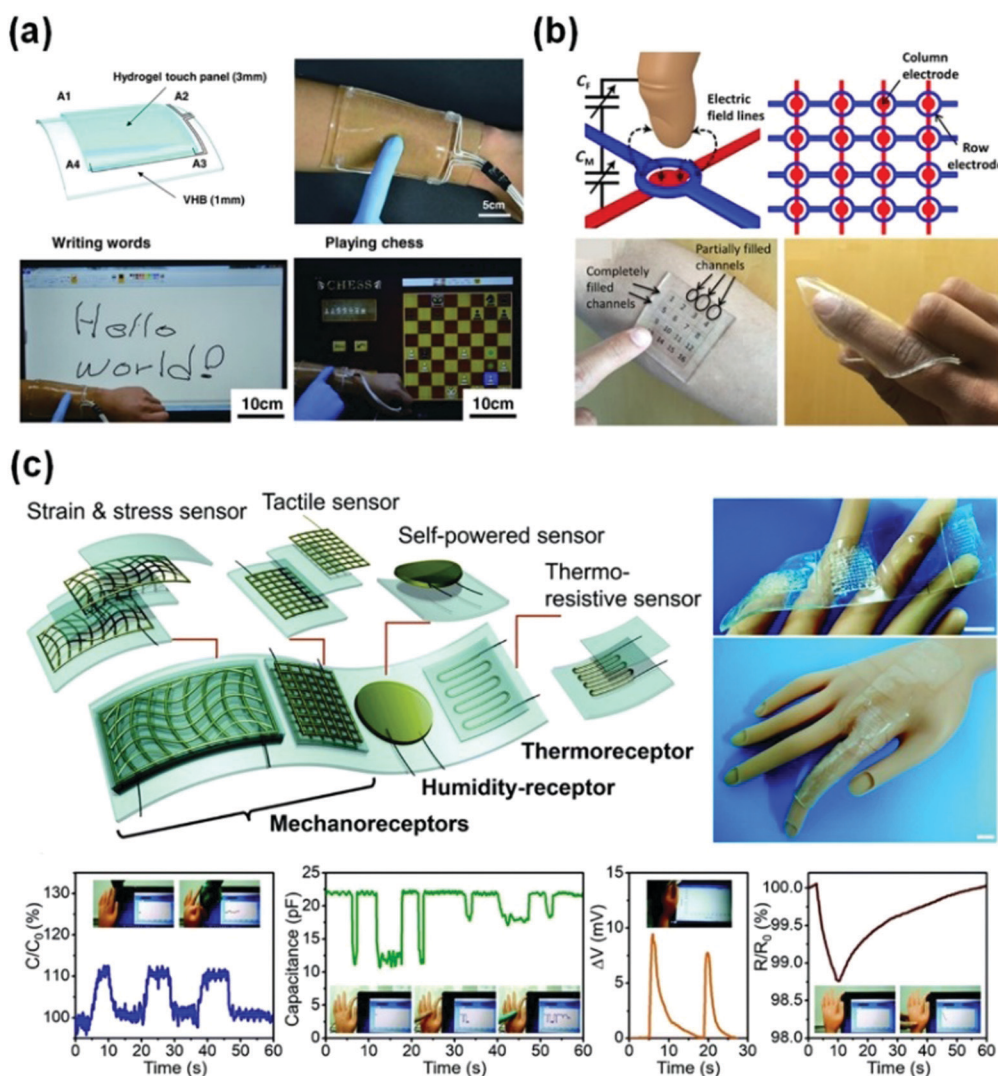
Fig. 14 Representative flexible devices based on conductive hydrogel sensors. (a) Wearable ionic hydrogel touch panels. Reprinted from ref. 220 with permission. Copyright 2016 AAAS. (b) A 4 \times 4 cross-grid sensor array. Reprinted from ref. 137 with permission. Copyright 2017 AAAS. (c) Integration of a strain and stress sensor, a tactile sensor, a self-powered sensor and a thermo-resistive sensor and receptors into single devices. Reprinted from ref. 153 with permission. Copyright 2019 Royal Society of Chemistry.
