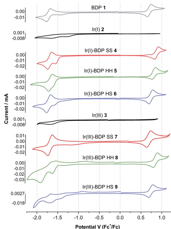
Fig. 7 Cyclic voltammograms of the parent compounds BDP 1, Ir(II) 2 and Ir(III) 3, and the bifunctional catalysts 4–9, measured in a 0.1 M solution of TBA- BAR_4^F in dichloromethane under argon. Ferrocene was used as internal standard. Scan rate: 100 mV s^{-1} .
