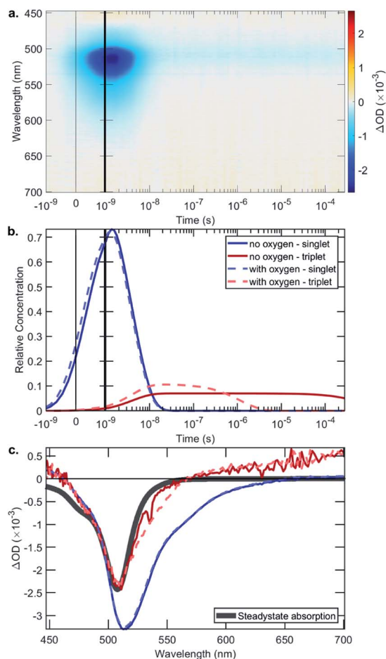
Fig. 6 The data from the transient absorption spectroscopy measurements for Ir(II)–BDP SS 4, chosen as a representative example: (a) the collected data, in the absence of oxygen, using an excitation wavelength of 355 nm; (b) fitted exponential decay showing the time dependent behaviour of the singlet and triplet excited states; and (c) the species associated spectra.
