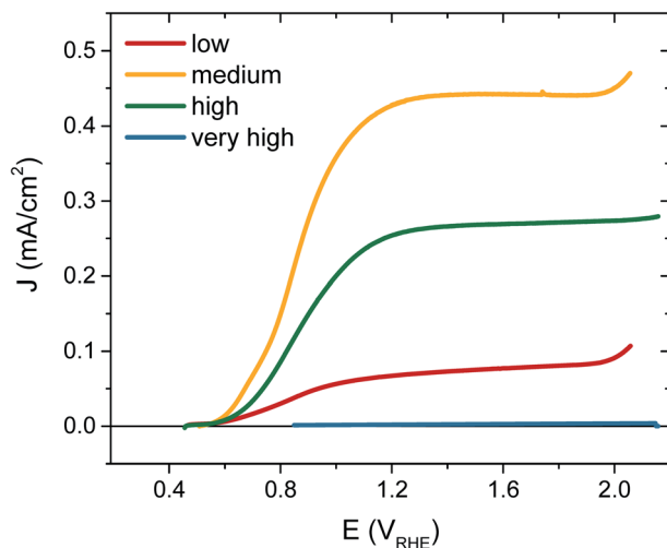
Fig. 3 Photocurrent responses for each \text{WO}_3 sample under simulated 1 sun illumination from the front side in 0.1 M \text{H}_2\text{SO}_4 , scan rate 10 mV \text{s}^{-1} . Data given for 'very high' [\text{V}_\text{O}] (blue), 'high' [\text{V}_\text{O}] (green), 'medium' [\text{V}_\text{O}] (yellow) and 'low' [\text{V}_\text{O}] (red).
