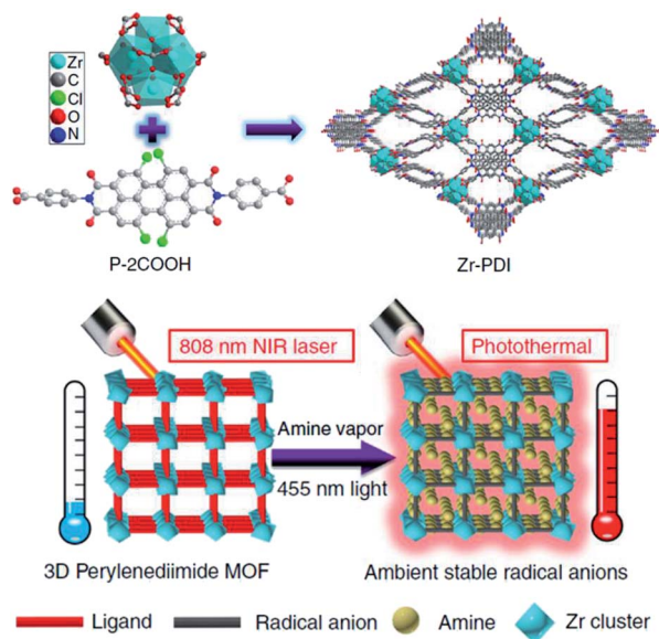
Fig. 9 The fabrication of Zr-PDI and Zr-PDI \cdot^- and their photothermal conversion abilities at 808 nm. Reproduced from ref. 55 with permission from Nature Publishing Group, Copyright 2019.
