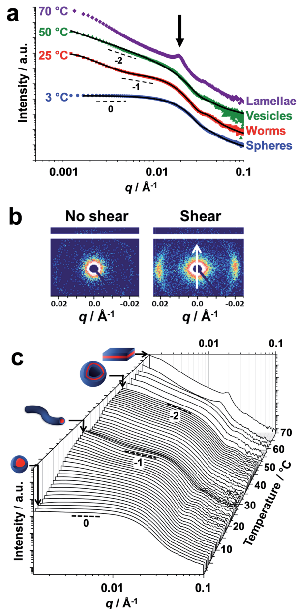
Fig. 4 Small-angle X-ray scattering studies of linear diblock copolymer nano-objects. (a) Double-logarithmic plot of SAXS patterns recorded for a 1.0% w/w aqueous dispersion of thermoresponsive PDMA 56 -P(HBA- stat -DAAM) 264 nano-objects at 3 °C (blue data), 25 °C (red data), 50 °C (green data) and 70 °C (purple data). The black lines indicate the data fits obtained using appropriate scattering models. For guidance, black dashed lines indicate zero, -1 and -2 gradients, while the blue, green and purple data sets are offset by arbitrary factors to aid clarity. (b) 2D SAXS patterns recorded either at zero shear or under applied shear (direction indicated by the white arrow) during rheo-SAXS experiments conducted on a 20% w/w aqueous dispersion of PDMA 56 -P(HBA- stat -DAAM) 264 nano-objects at 63 °C. (c) SAXS patterns recorded for a 1.0% w/w aqueous dispersion of thermoresponsive PDMA 56 -P(HBA- stat -DAAM) 264 nano-objects between 1 and 70 °C using a heating rate of 1 °C min -1 . For guidance, black dashed lines indicate zero, -1 and -2 gradients.
