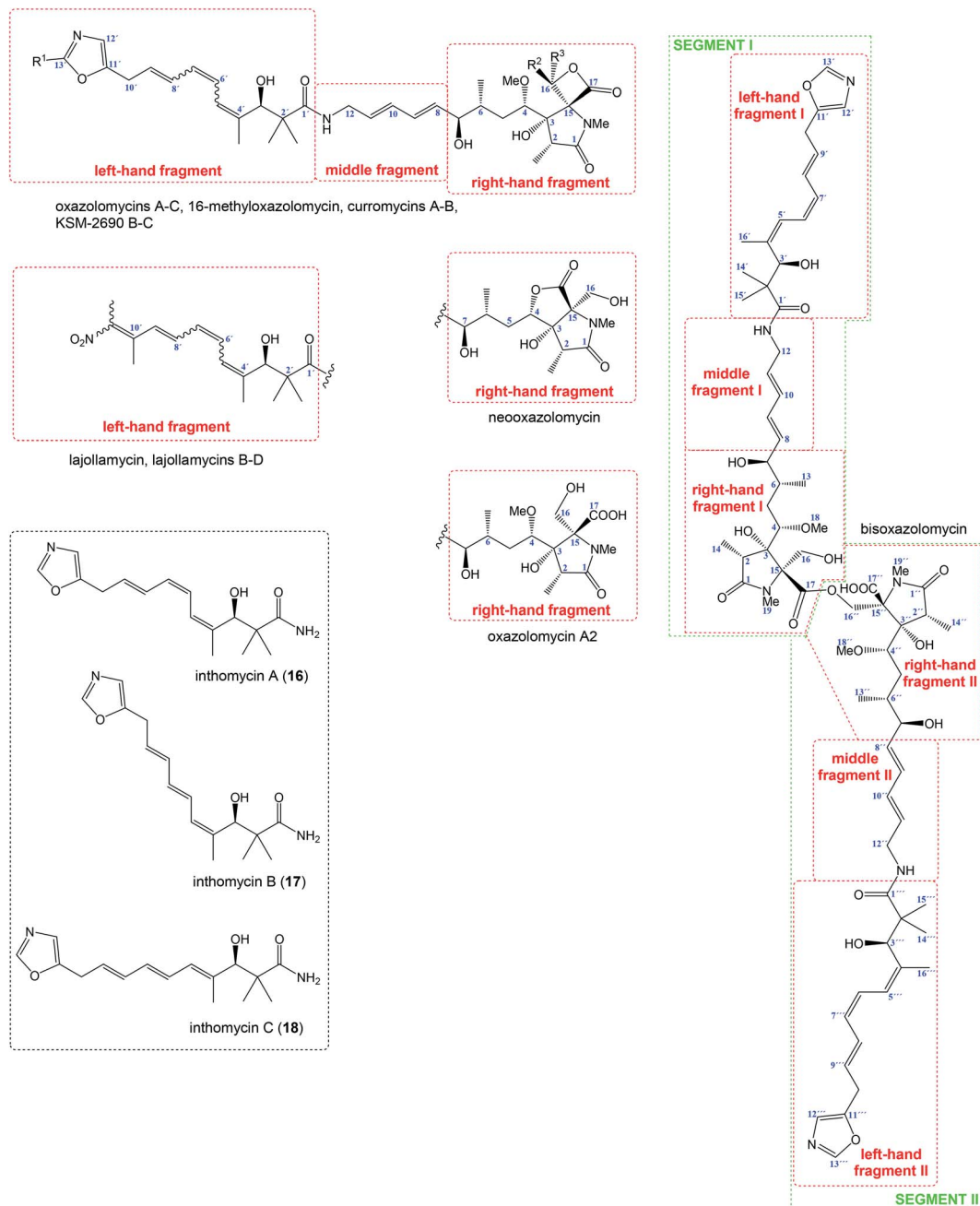
Fig. 2 Structural division of oxazolomycin family members and structure of inthomyicins.
