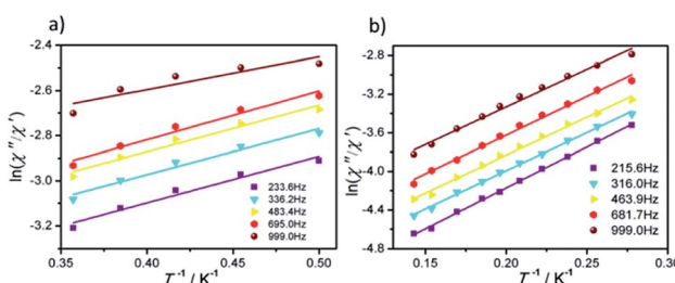
Fig. 6 Plots of \ln(\chi''/\chi') vs. 1/T for 1 (a) and 2 (b) under 0 Oe dc field, the solid lines represent the best fits.
