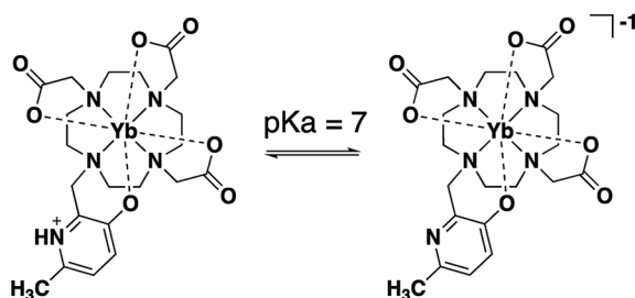
Scheme 1 Deprotonation of HMP in Ln(III) -DO3A-HMP between pH 6 and pH 8 increases the electron density of the coordinating oxygen, perturbing the ligand field, and leading to an enhanced change in the NMR shift of the pyridyl methyl group over a diamagnetic analog due to the shifting pseudocontact field of the lanthanide.
