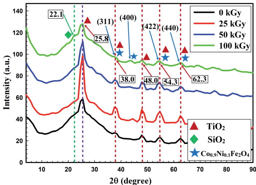
Fig. 5 XRD pattern showing the effect of gamma irradiation, with doses of 25, 50 and 100 kGy, on the crystal size of the prepared Co x Ni 1-x Fe 2 O 4 /SiO 2 /TiO 2 ; x = 0.9 nanocomposite, compared with the non-irradiated composite.
