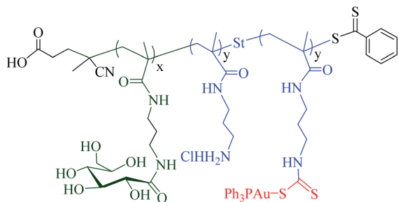
Fig. 8 Chemical structures of glycopolymer-based gold(I) phosphines DTC-conjugates (37).
