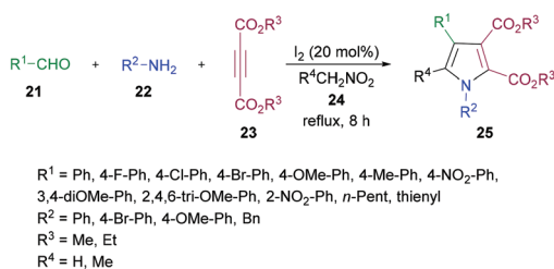
Scheme 5 Iodine-catalyzed four-component synthesis of tetrasubstituted pyrroles from aldehydes, amines, alkynoates and nitromethane.
