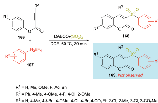
Scheme 40 Synthesis of 3-sulfonated coumarins from aryl propiolates and aryldiazonium tetrafluoroborates in the presence of DABSO.
