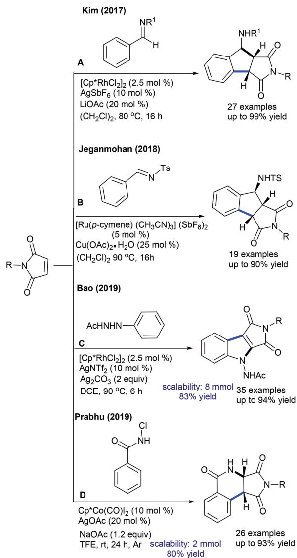
Scheme 88 Synthesis of 1-aminoidanes/fused heterocycles.
