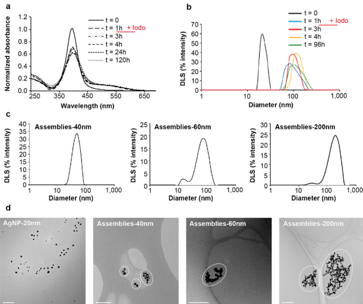
Fig. 2 AgNP assemblies: production, purification and characterization. (a) Time-dependent analysis of AgNP SPR spectra in the presence of \text{L}^{35} between 0 and 120 hours of incubation at a S : Ag molar ratio of 0.25 : 1. The reaction between AgNPs and \text{L}^{35} occurs for 1 hour, then iodoacetamide is added at 100 \mu\text{M} for a thiol concentration of 90 \mu\text{M} . SPR spectra were acquired up to 120 hours of the total incubation time. (b) In a set-up similar to (a), hydrodynamic diameter distribution of the species in solution was determined for the AgNPs alone ( t = 0 ), at t = 1\text{h} (time for the addition of iodoacetamide) and then at t = 3, 4 and 96 hours. (c) Hydrodynamic diameter distribution of different populations of assemblies separated by discontinuous sucrose gradient centrifugation. Three different populations were recovered: "Assemblies-40 nm" corresponds to assemblies of 40 nm average diameter by DLS, "Assemblies-60 nm" corresponds to assemblies of 60 nm average diameter by DLS and "Assemblies-200 nm" corresponds to assemblies of 200 nm average diameter by DLS. (d) Analysis by cryo-TEM of the different populations of assemblies compared to initial AgNPs, for which a proper dispersion on the grid is obtained. Assemblies composed of a larger number of particles with a larger diameter of the assemblies were observed on the grids. Clusters of AgNPs considered as an assembly are encircled to help the understanding of our statistical analysis (Fig. S4b, ESI†). The scale bar corresponds to 200 nm. "Iodo" stands for iodoacetamide.
