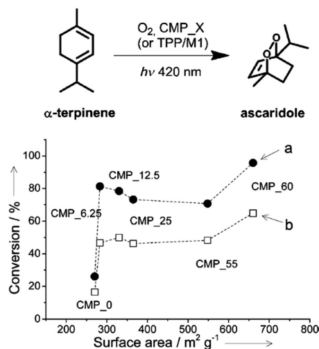
Fig. 17 Porosity control of CPPs by the silica template. Photocatalytic conversion of \alpha -terpinene into ascaridole with poly(benzothiadiazole)s having different surface areas. Photo-reactor set-up with (a) lower O_2 flow rate (5 mL min^{-1} ) and (b) higher O_2 flow rate (10 mL min^{-1} ). Adapted with permission. 22 Copyright 2013 Wiley-VCH.
