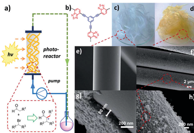
Fig. 21 Processing of CPPs for a flow column photo-reactor. (a) Schematic set-up of a fixed-bed flow photo-reactor with CPP-coated glass fibers. (b) The chemical structure of photoactive CPP. Photographs of (c) pure glass fiber and (d) CPP-coated glass fiber. SEM images of (e) pure glass fiber and (f–h) CPP-coated glass fiber. Adapted with permission. 37 Copyright 2017 The Royal Society of Chemistry.
