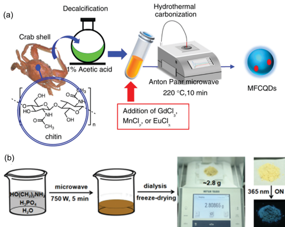
Fig. 5 (a) Schematic illustration of preparation of C-dots by a microwave-assisted approach. (b) Schematic illustration of the preparation process for C-dots with a gram scale product. Right side of (b): the purified C-dot powder under daylight and a 365 nm ultraviolet (UV) lamp. (a) Reproduced with permission from ref. 98. Copyright 2017, American Chemical Society. (b) Reproduced with permission from ref. 69. Copyright 2018, Wiley-VCH.
