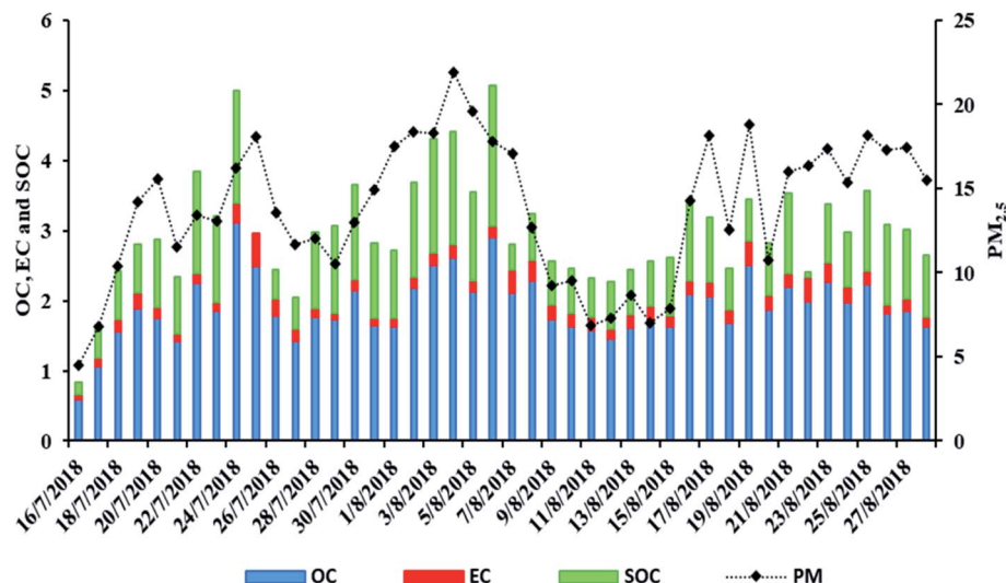
Fig. 2 Daily variations of PM_{2.5} , OC, EC and SOC ( \mu g m^{-3} ) of samples collected at AGM.
