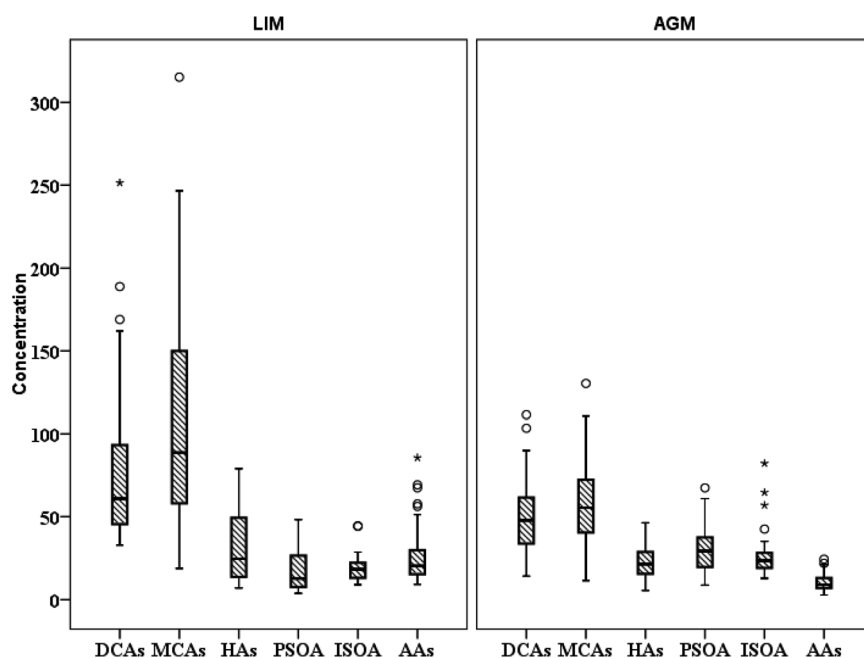
Fig. 3 Spatial distribution of the sum of studied polar organic compound groups ( ng m^{-3} ) (○ refers to values above the 3 rd quartile and * to outliers).
