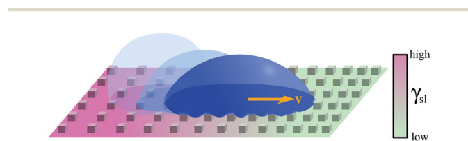
Fig. 6 Simplified schematic of droplet transport due to gradients in surface texture. Space-varying structural features can lead to directional droplet transport at a velocity \mathbf{v} towards areas of lower surface energy by influencing the contact angle that the droplet assumes on it. For example, an array of pillars of varying width and separation can induce a droplet to move towards areas of larger surface coverage when contact angle hysteresis is overcome. 7
